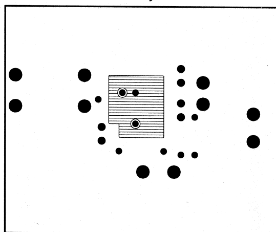
Inner Layer Ground
